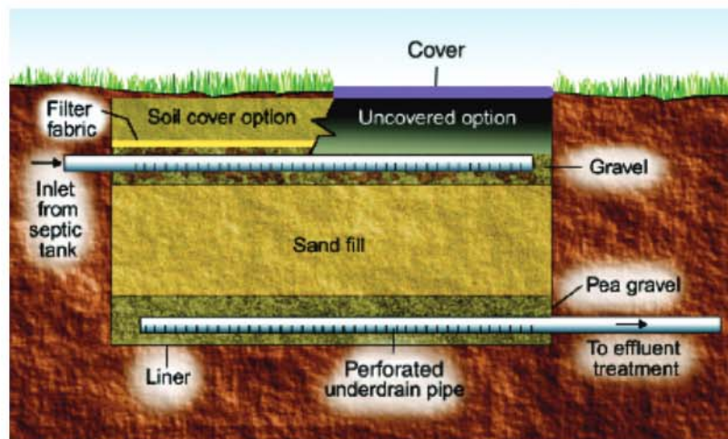
Figure 6: Sand filter.
