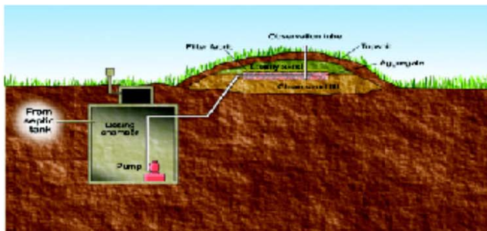
Figure 5: Mound system.
