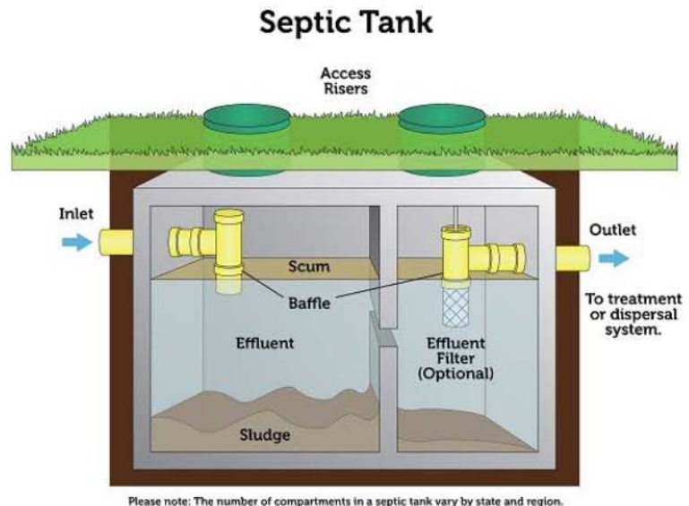
Figure 2: Septic tank.
